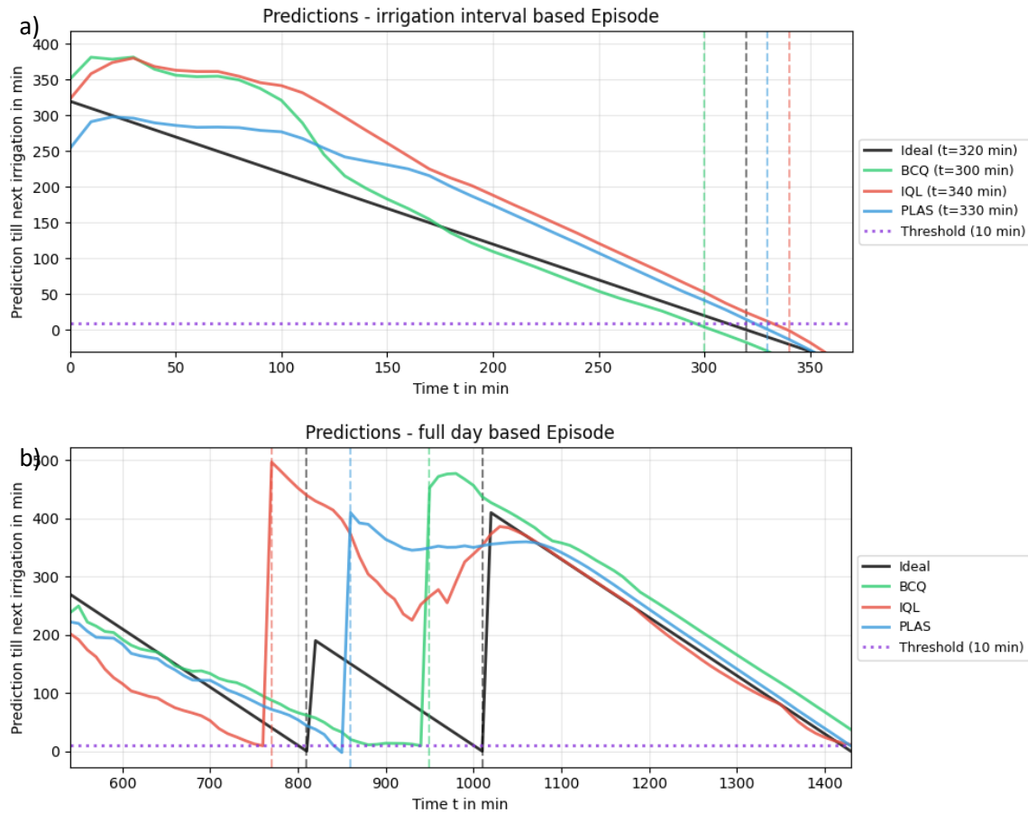
Figure 5: Example episodes showing the predicted action over time for three offline RL policies (BCQ, IQL, PLAS) compared to the ideal irrigation schedule. a) for the irrigation interval based Episode and b) for the full day based Episode. The solid black curve indicates the ideal action and the colored curves correspond to the respective policy predictions. The vertical dashed lines indicate when each policy would irrigate.
